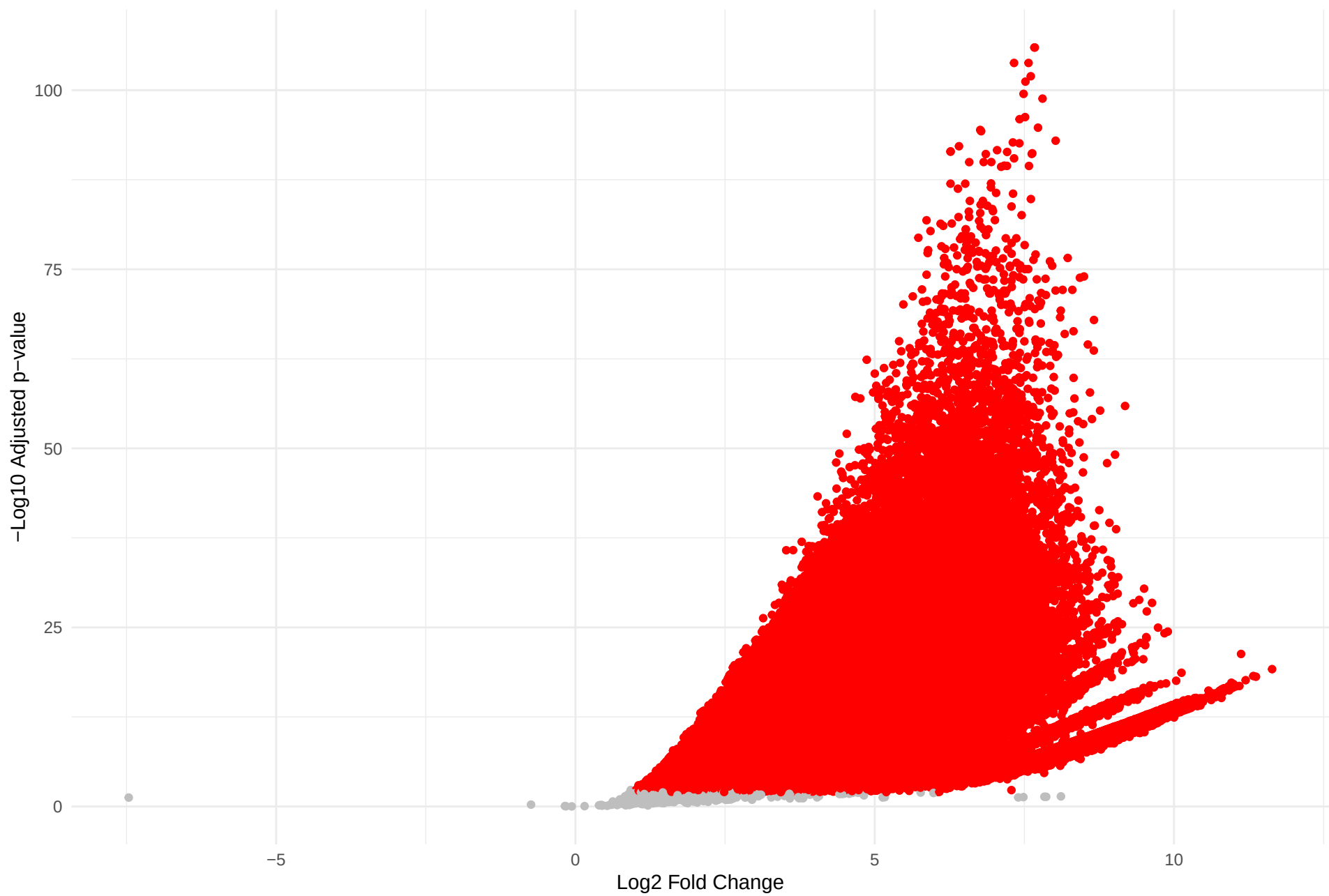
DMSO_Chromatin vs DMSO_Cytoplasm
